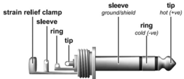
Fig .4.5: 1/4" TRS connector
